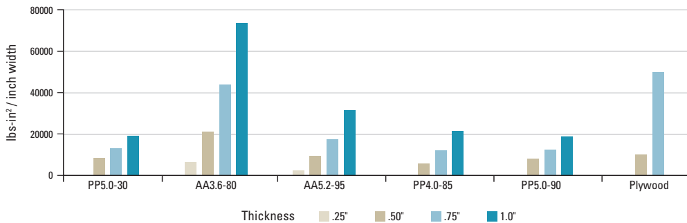
Aluminum Honeycomb 3.6 pcf with .020" Aluminum
