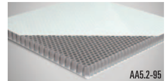
Aluminum Honeycomb 5.2 pcf with 0.18" Glass-Epoxy
