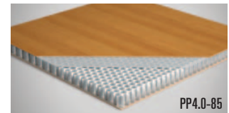
PP Honeycomb 4.0 pcf with .059" Okume Plywood
