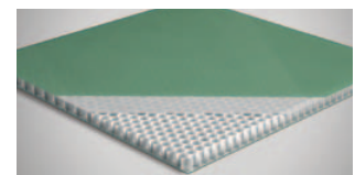
PP Honeycomb 5.0 pcf with .014" Glass-Epoxy with Peel Ply
