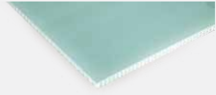
PP5.0-90 PP Honeycomb core 5.0 pcf with 0.014" Glass-Epoxy with Peel Ply film skin
